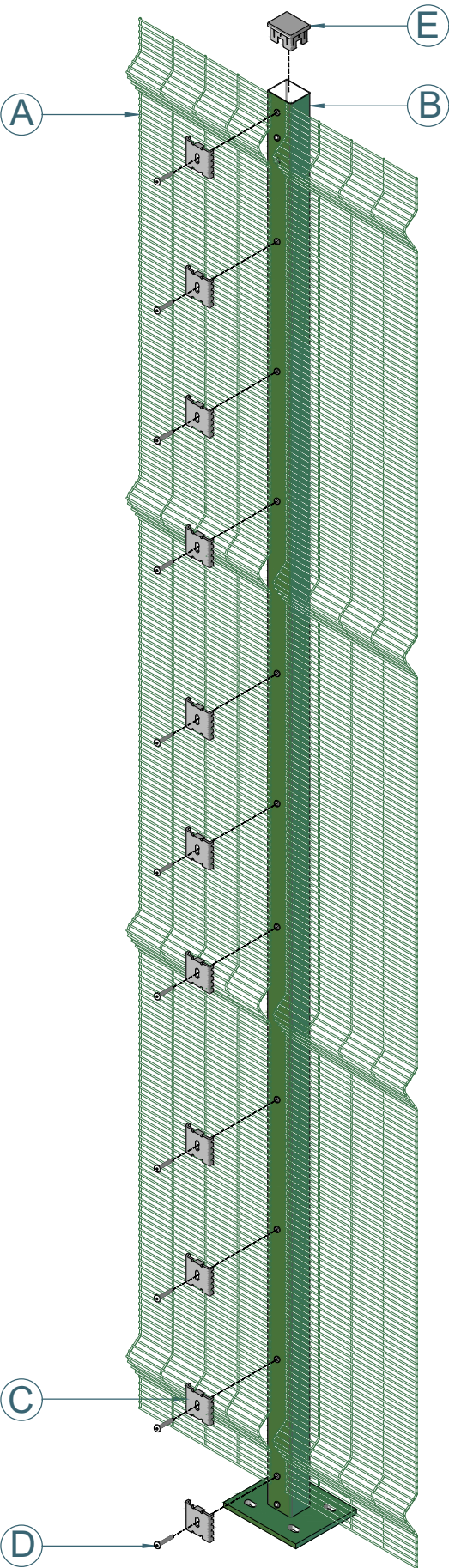
Axonometric Drawing
