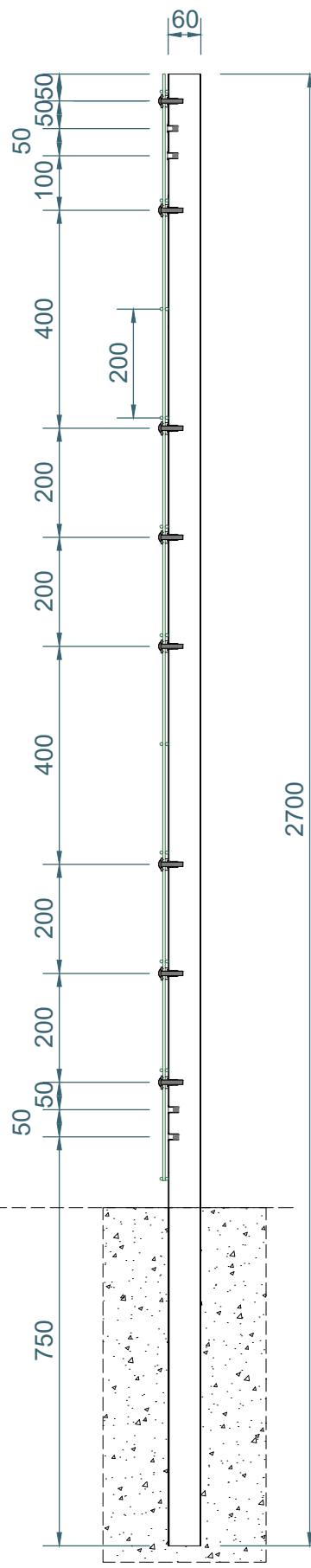
2-2 Section 1:12
