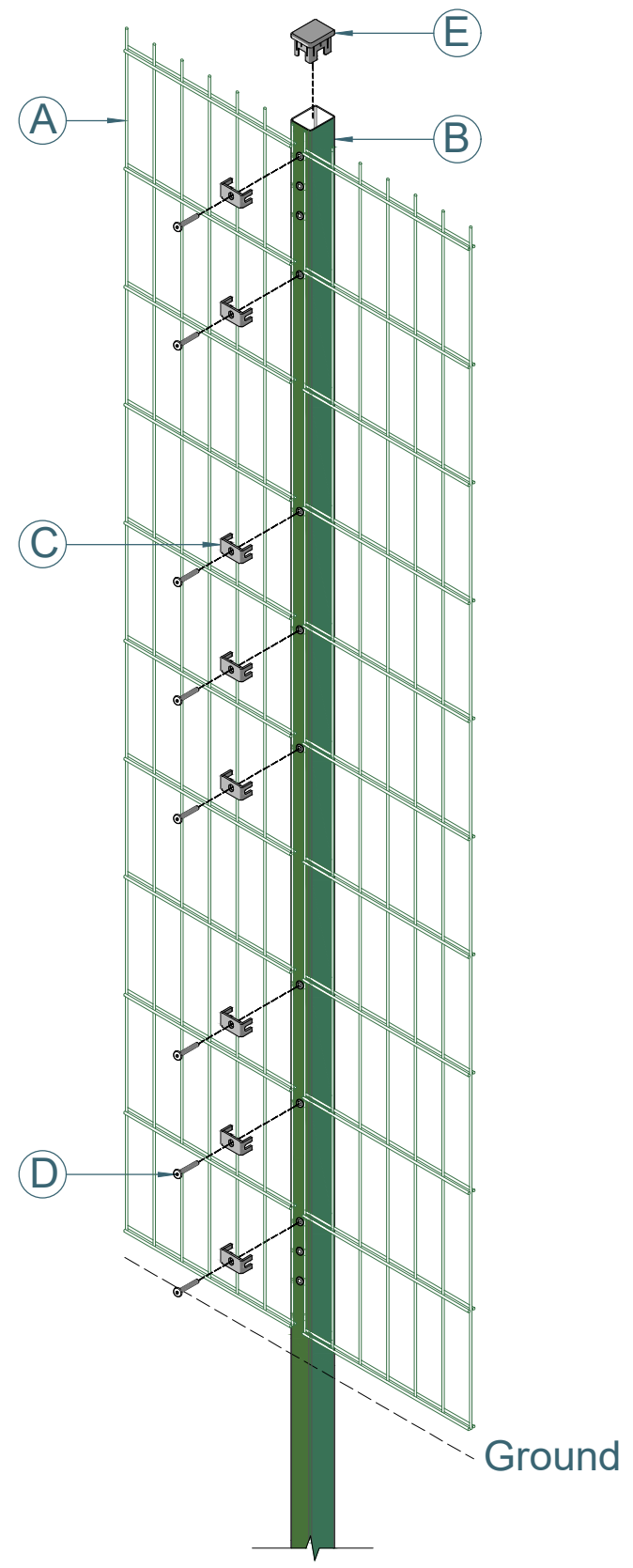
Axonometric Drawing
