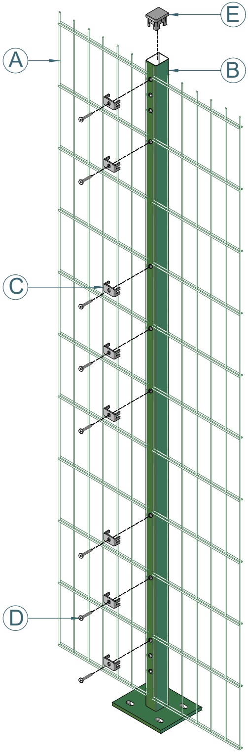
Axonometric Drawing
