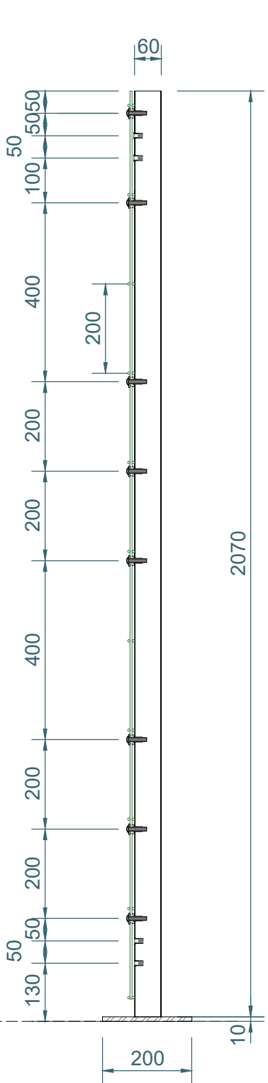
2-2 Section 1:12
